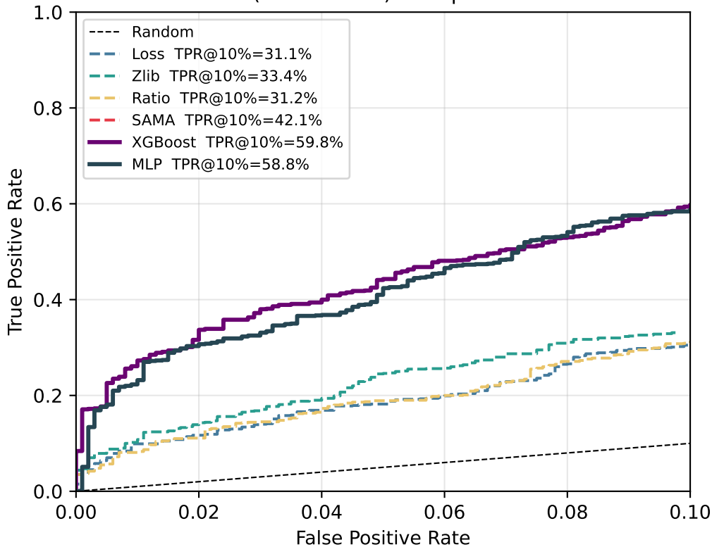
ROC (FPR \leq 10\% ) — Experiment 2
