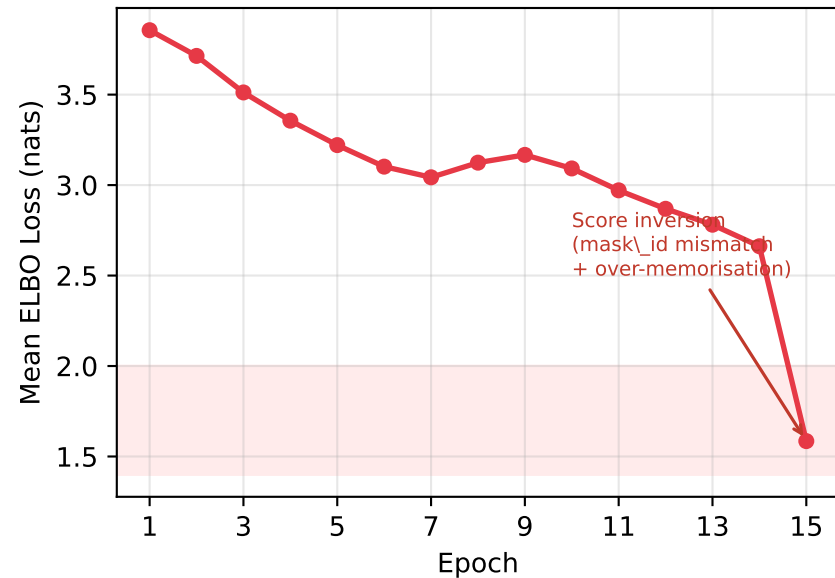
Experiment 1 (15 epochs, 45 eff. passes)
