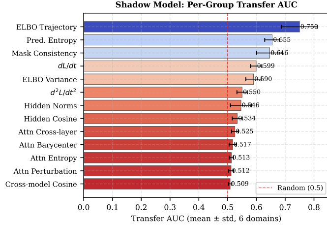
Figure 10: Per-group shadow transfer AUC (mean \pm std across six domains). ELBO trajectory is the only group that transfers above 0.70. All attention groups sit near 0.50.
