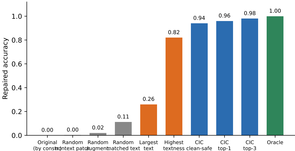
Failure-conditioned repair on 50 verified shortcut failures
