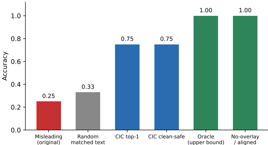
Hard multi-decoy held-out benchmark (OpenCLIP ViT-B-32)
