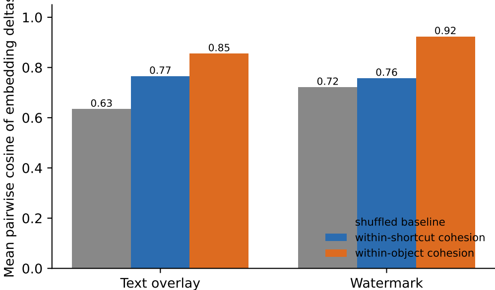
Object-entanglement: shortcut shift clusters by object, not shortcut value
