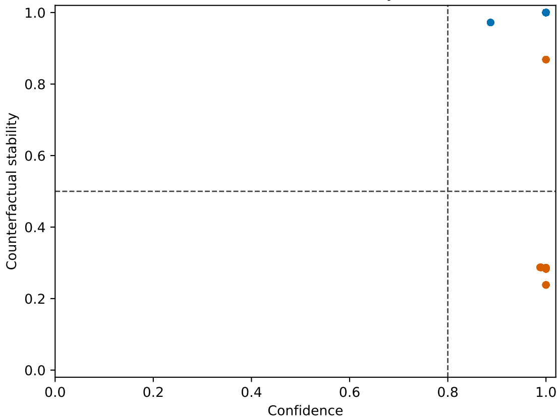
Real Text Shortcut Reliability Plane
