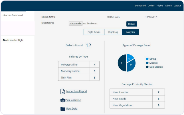
Inspection analytics — defects by type, damage classification, and proximity metrics.
