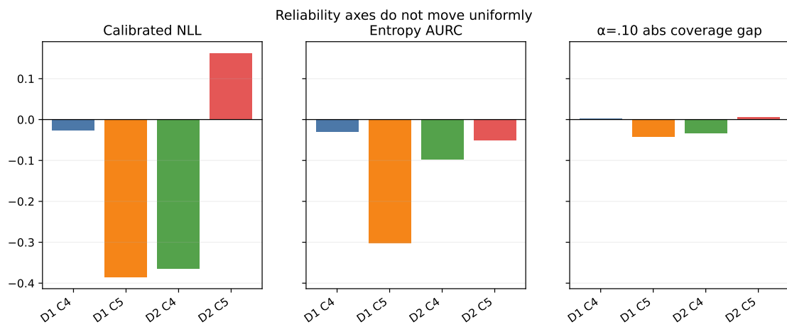
Figure 4: Paired effects across reliability axes.
