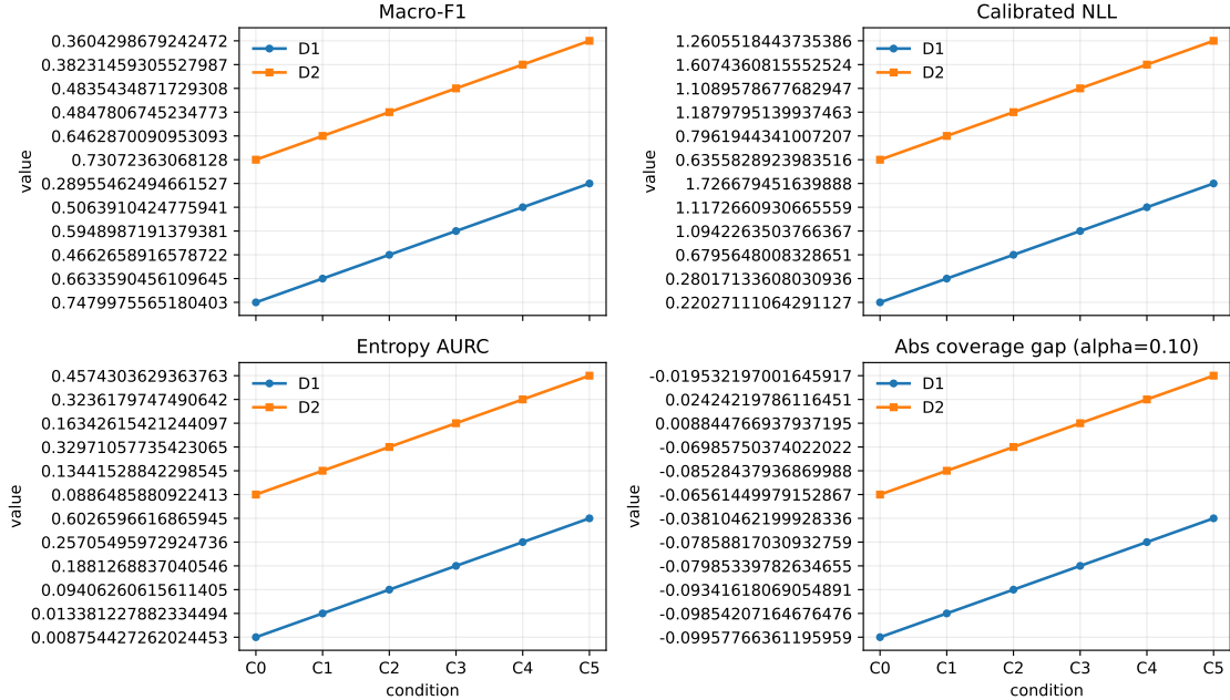
Figure 2: Canonical B0 v1.2 primary results across C0–C5. This manuscript-specific rendering replaces the earlier frozen presentation because its source-data audit found the original macro-F1 panel unavailable in the figure source.
