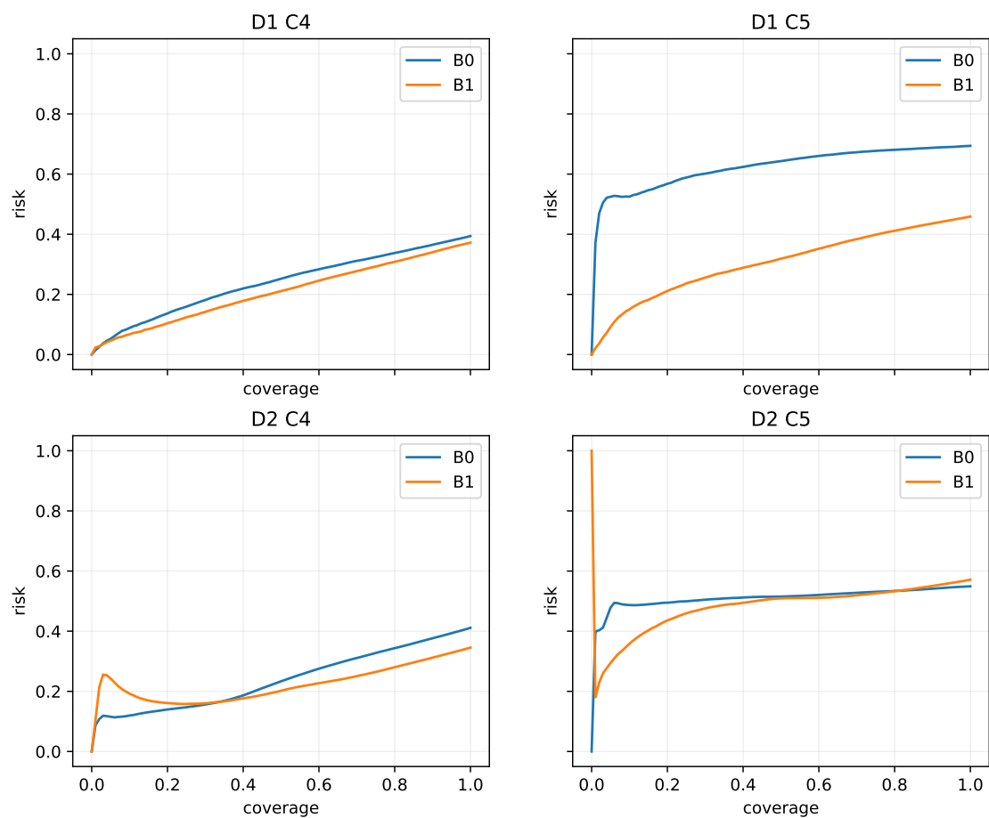
Figure 6: Representative frozen risk-coverage curves.
