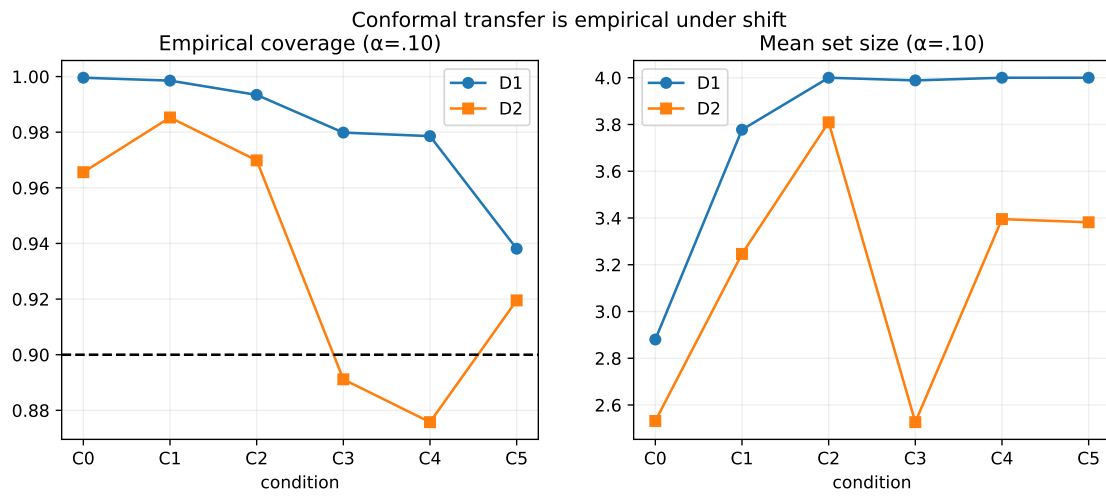
Figure 7: Empirical conformal coverage and mean set size under transfer.
