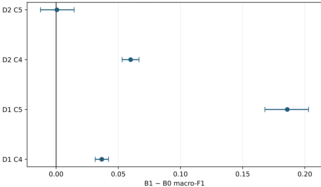
Compound predictive robustness
