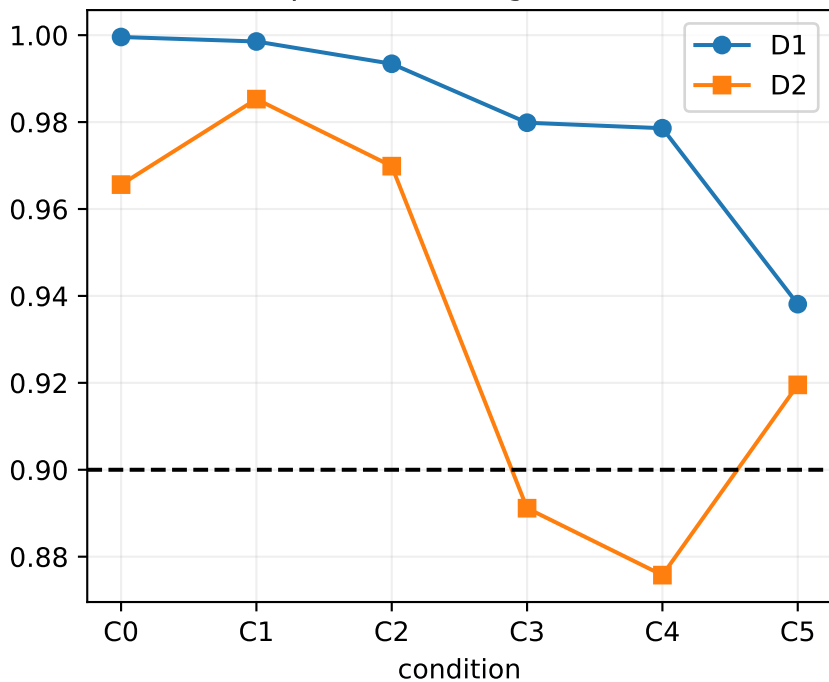
Empirical coverage ( \alpha=.10 )
