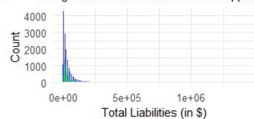
Histogram of TotalLiabilities vs Loan Approved
