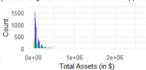
Histogram of TotalAssets vs Loan Approved
