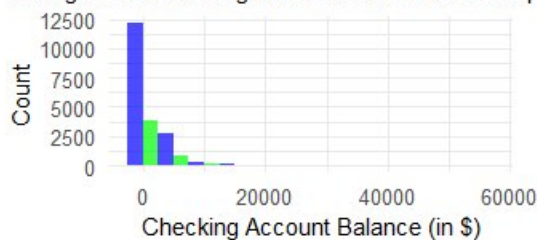
Histogram of CheckingAccountBalance vs Loan Approved
