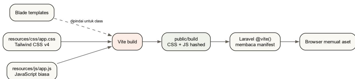
Gambar 2.2 Proses build Blade, Tailwind, JavaScript, dan Vite
