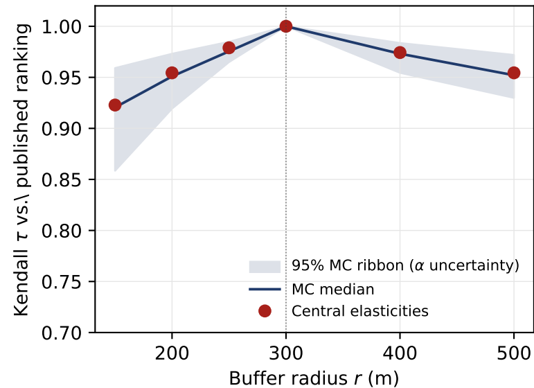
Ranking agreement under buffer-radius sweep
