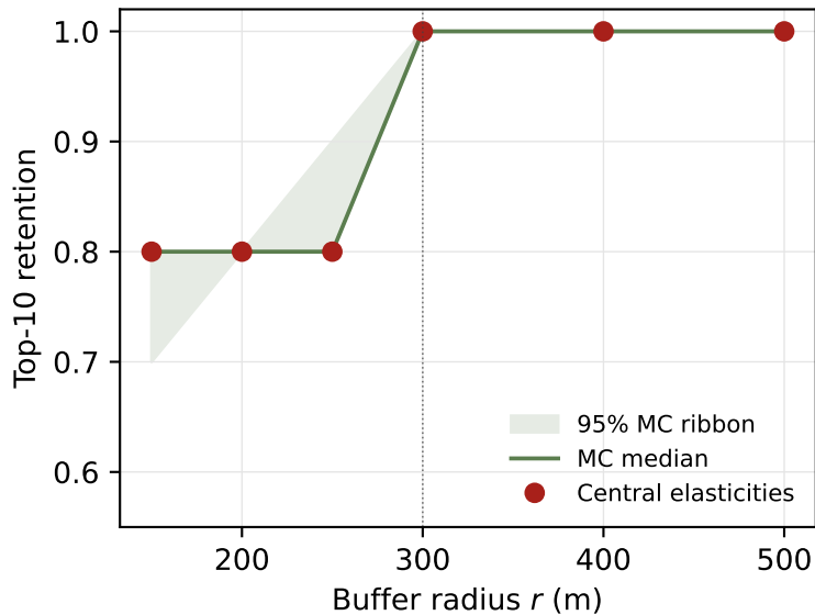
Top-10 retention under buffer-radius sweep
