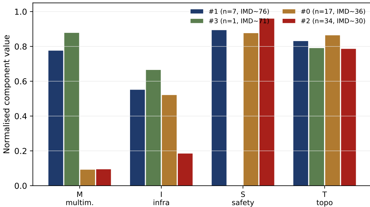
k-means archetypes of the dock-based panel (k=4)
