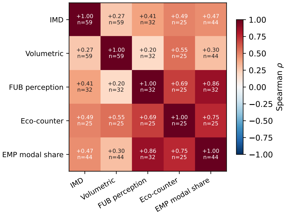
Inter-metric Spearman correlation
