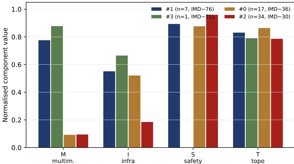
k-means archetypes of the dock-based panel (k=4)
