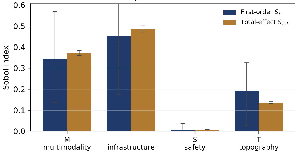
Variance decomposition of the IMD ( \delta = \pm 0.10 )
