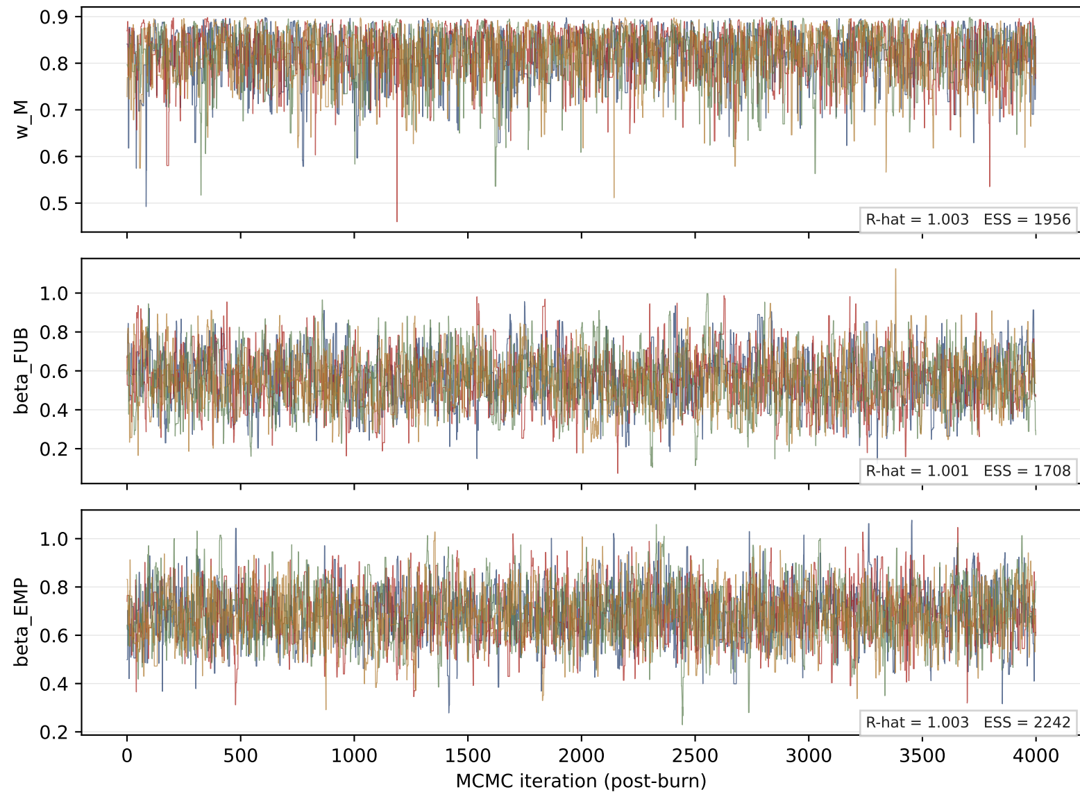
B4: trace plots over four MH chains
