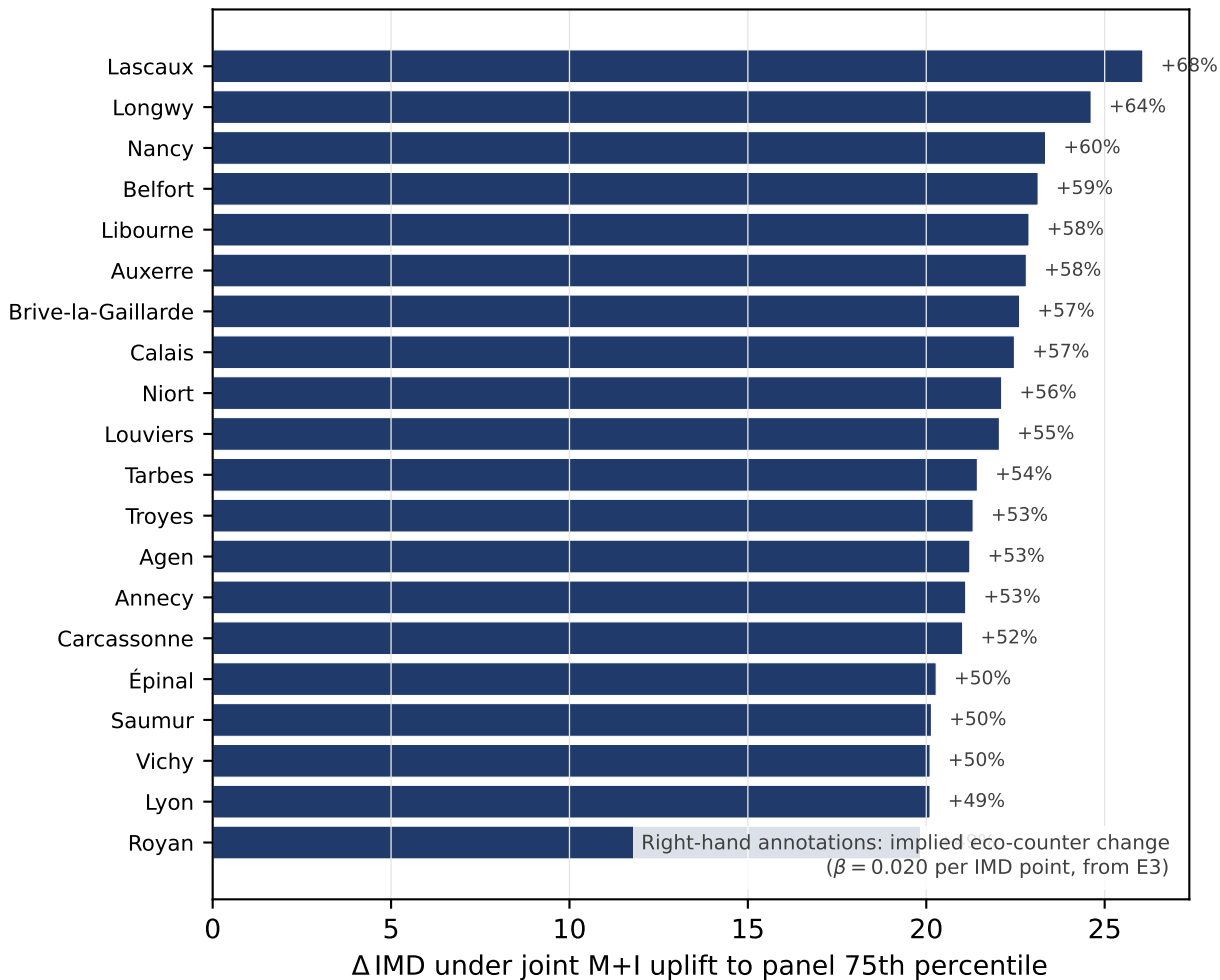
Top-20 cities by counterfactual uplift potential
