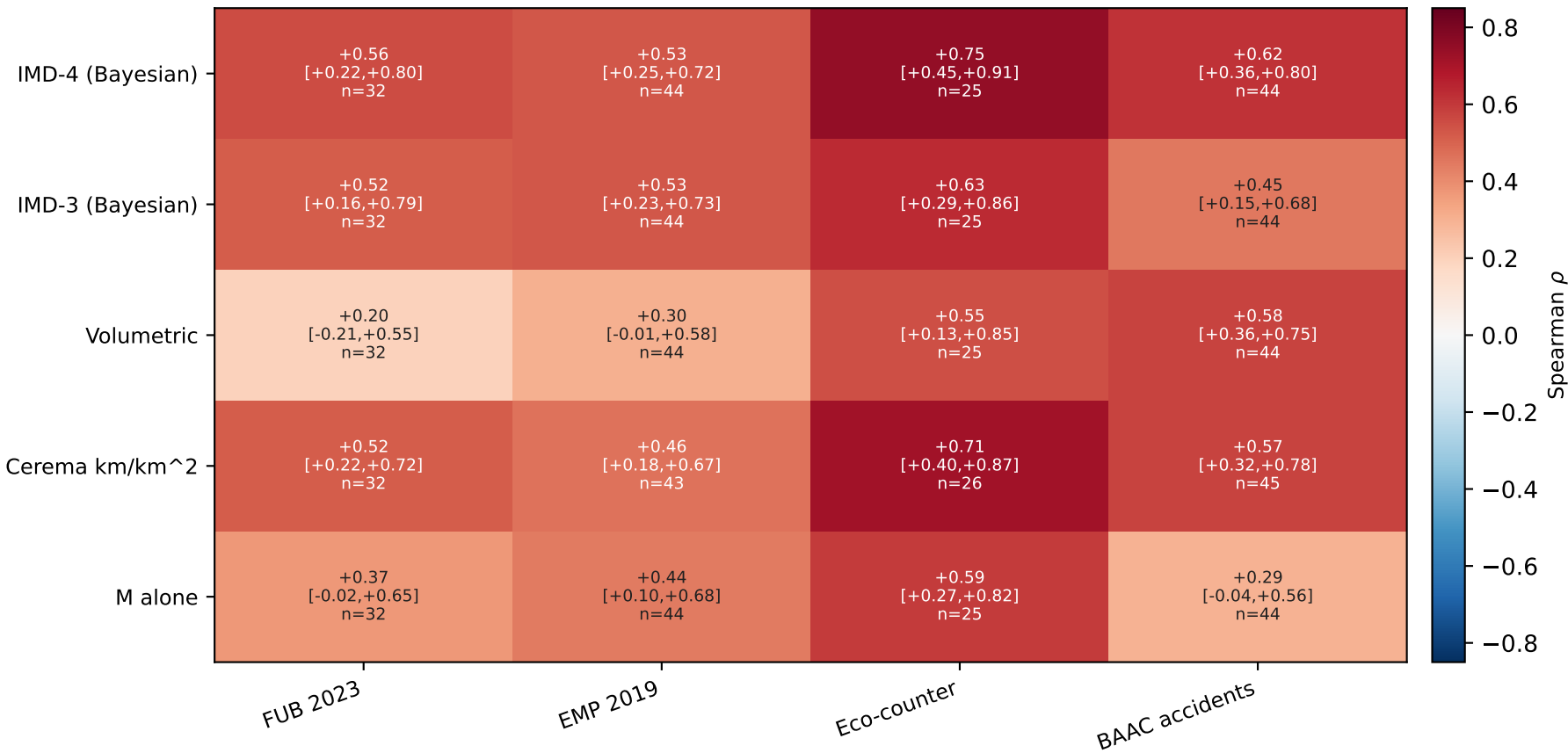
B13: Tournament with 1000-boot 95% CI on \rho
