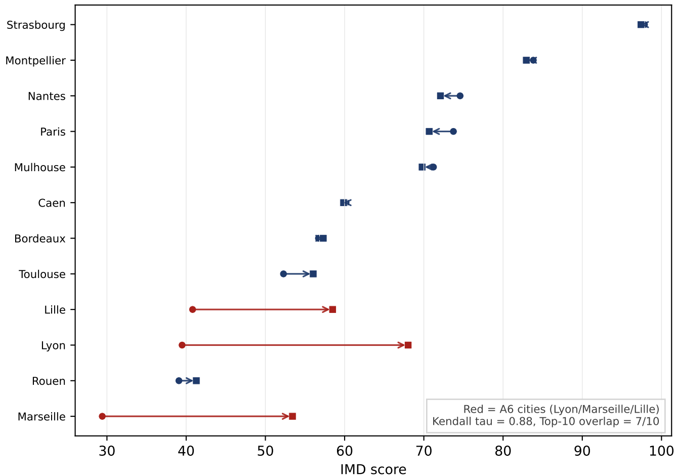
E30: IMD shift under A6 triangulation M = \max(C_M^{\text{GTFS}}, C_M^{\text{OSM}})
