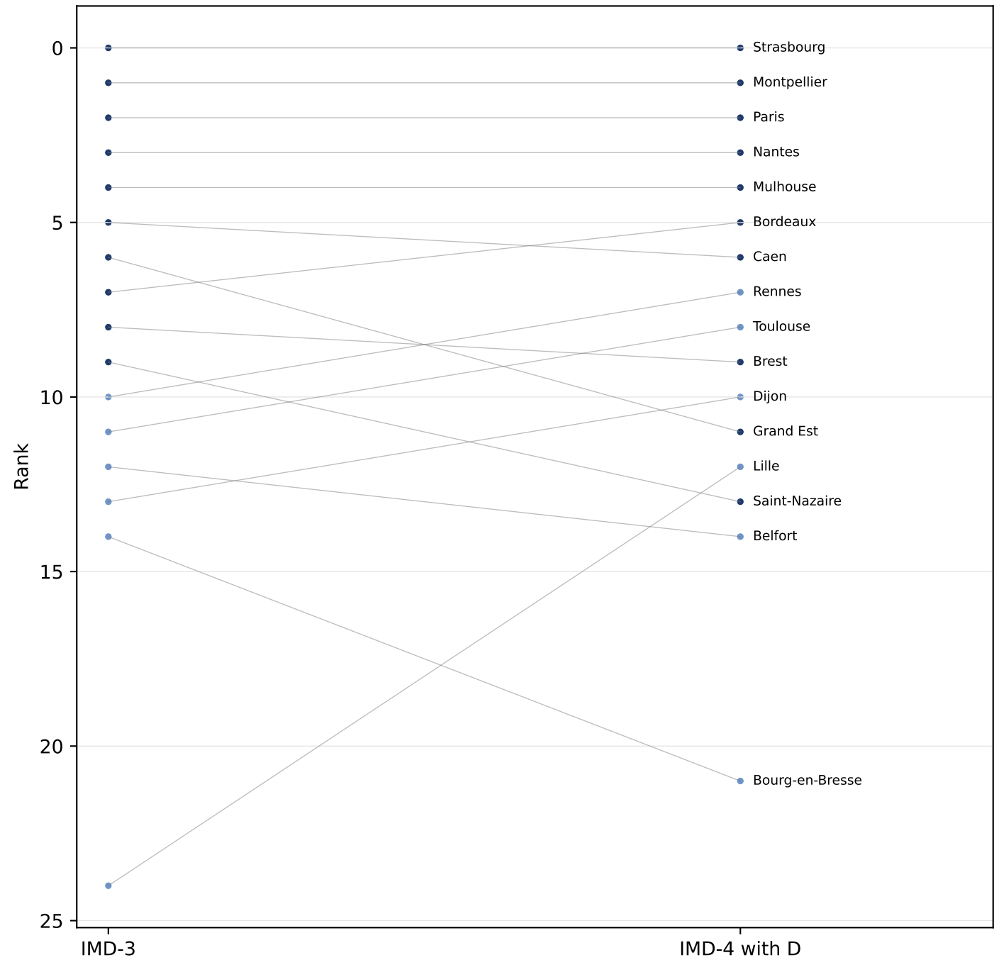
Ranking shift after adding population density (Top-15 union)
