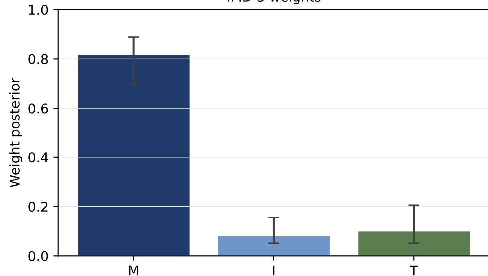
IMD-3 weights
