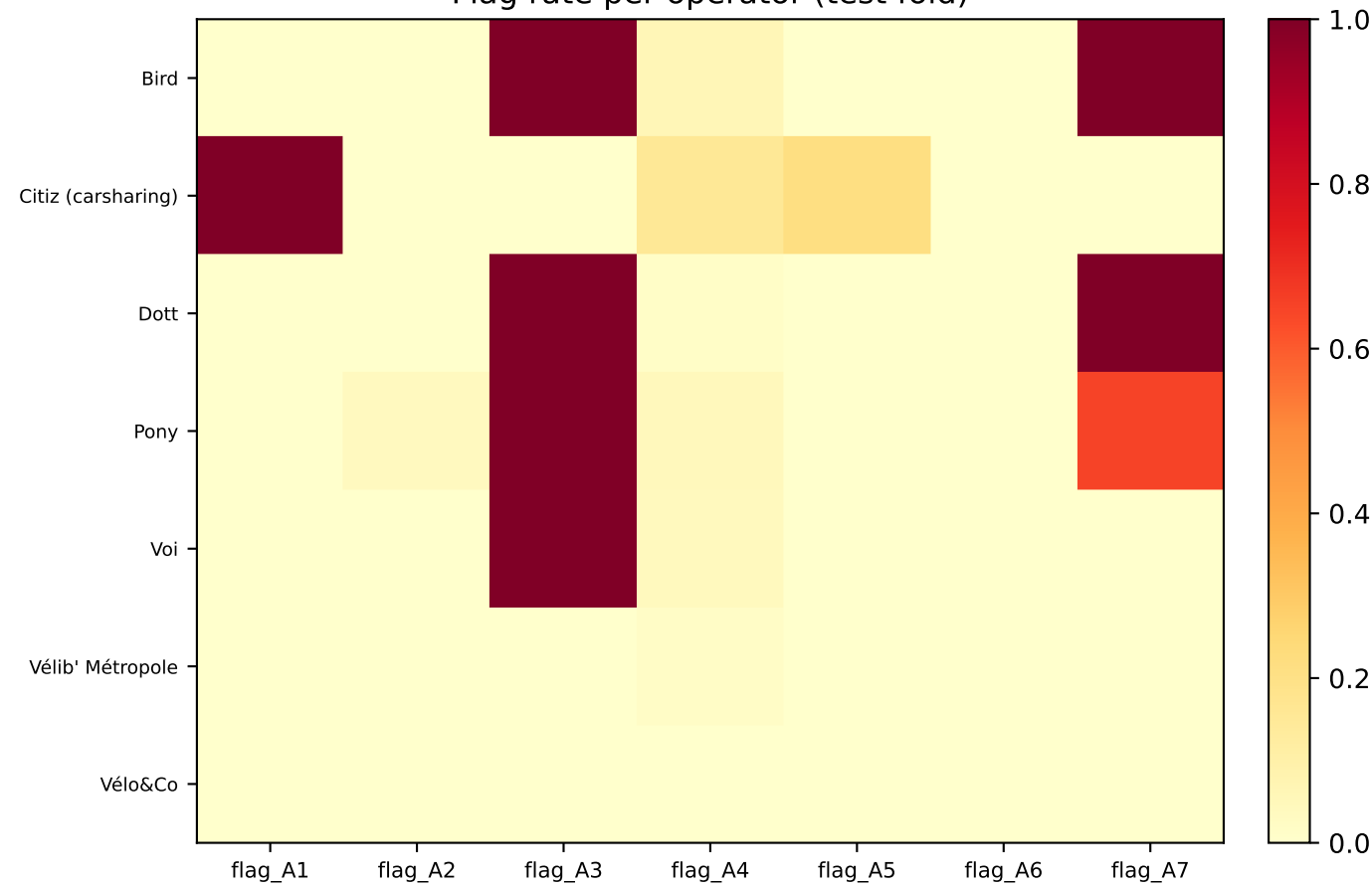
Flag rate per operator (test fold)
