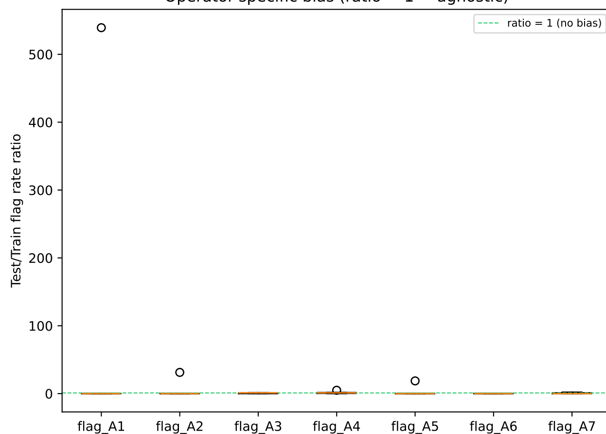
Operator-specific bias (ratio \approx 1 = agnostic)
