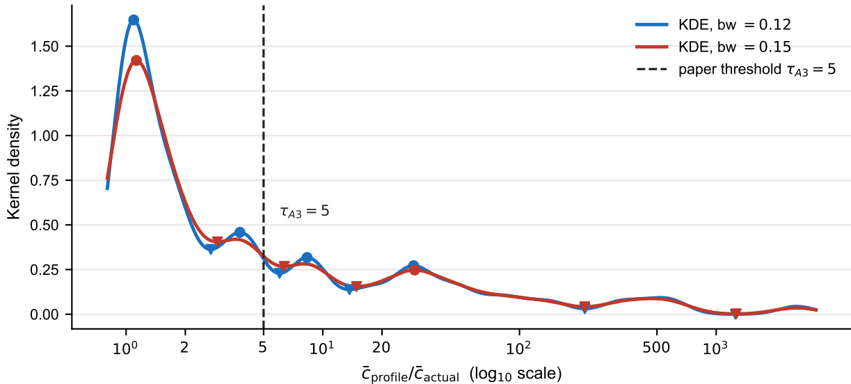
A3 ratio distribution on the global subset ( n = 98 , ratio > 1.01 )
