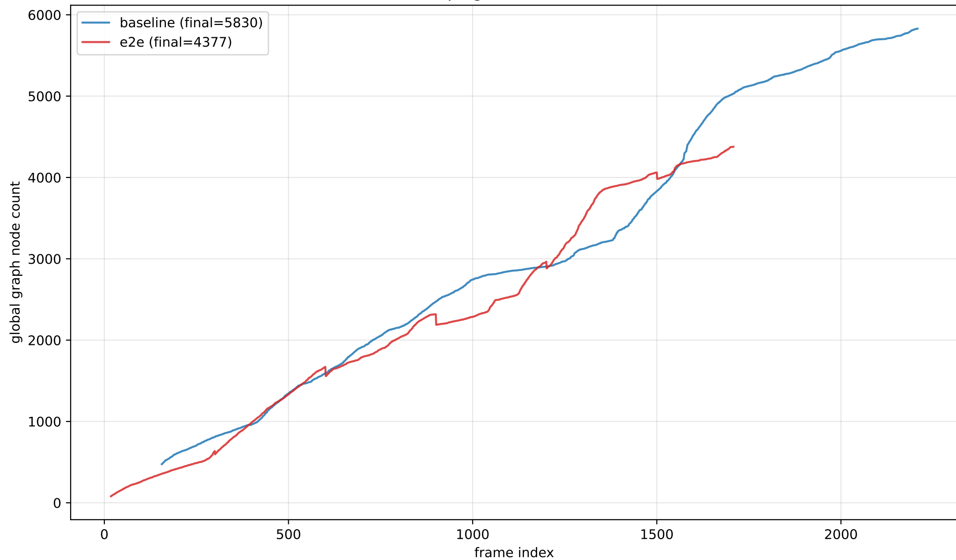
Graph growth over time
