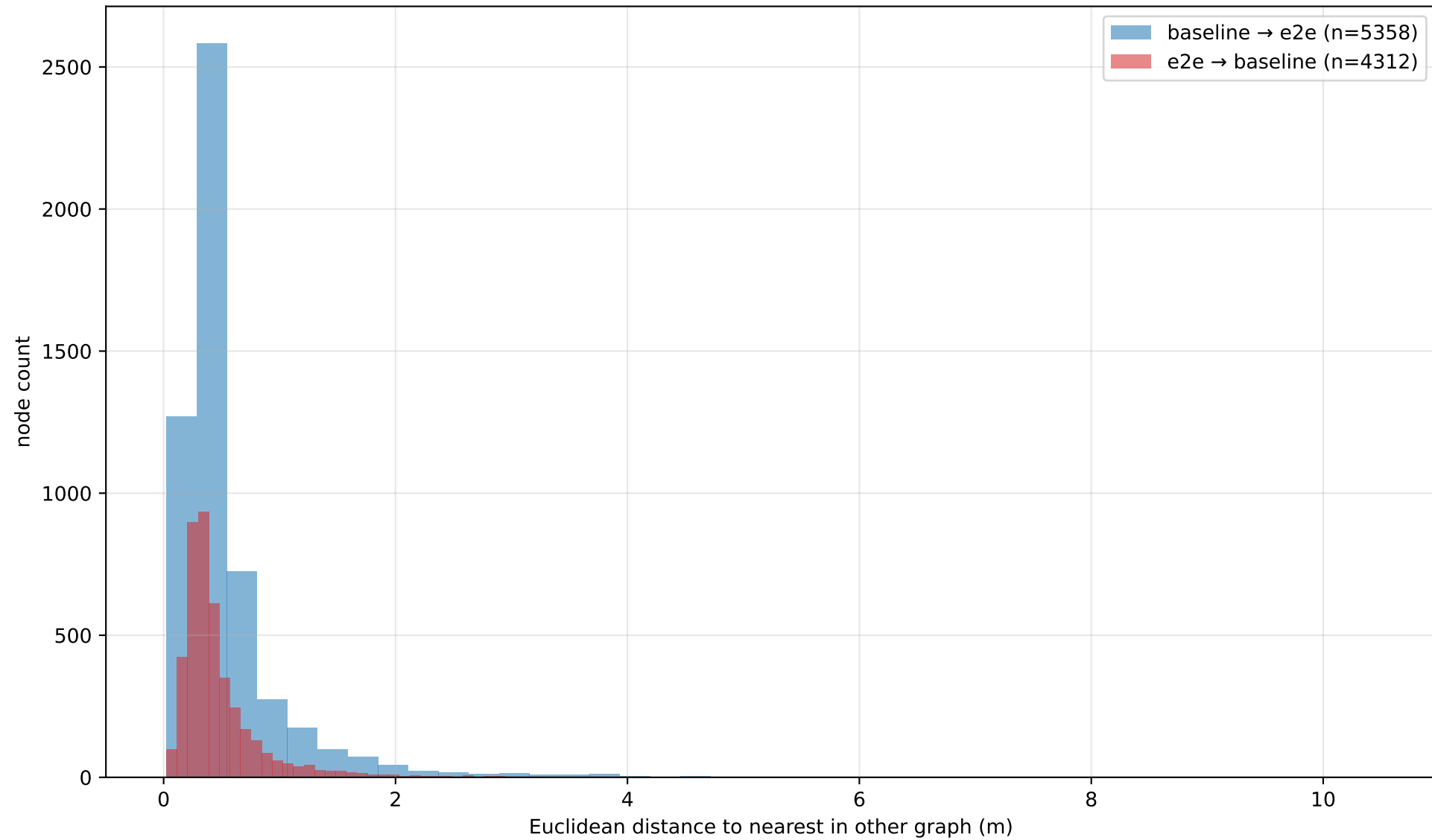
Nearest-neighbour distance distribution
