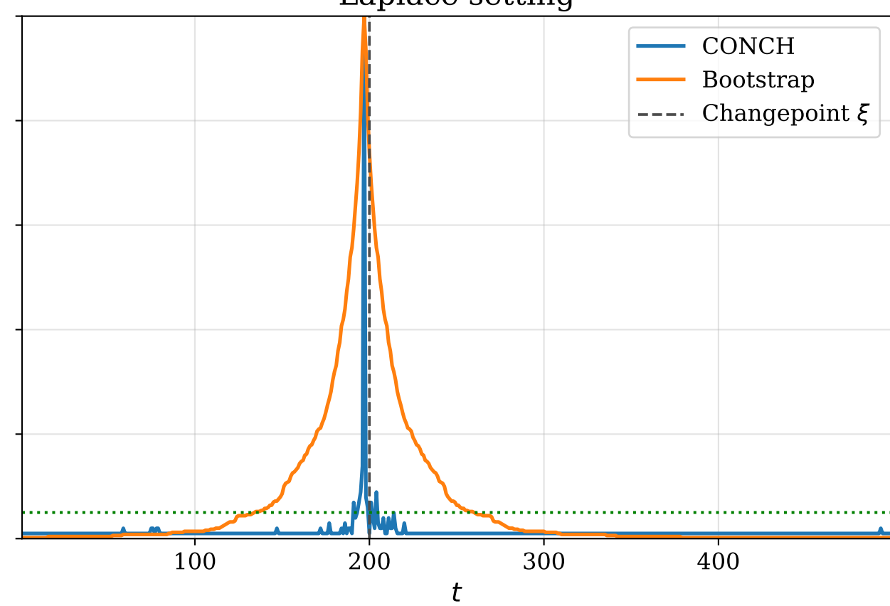
Laplace setting
