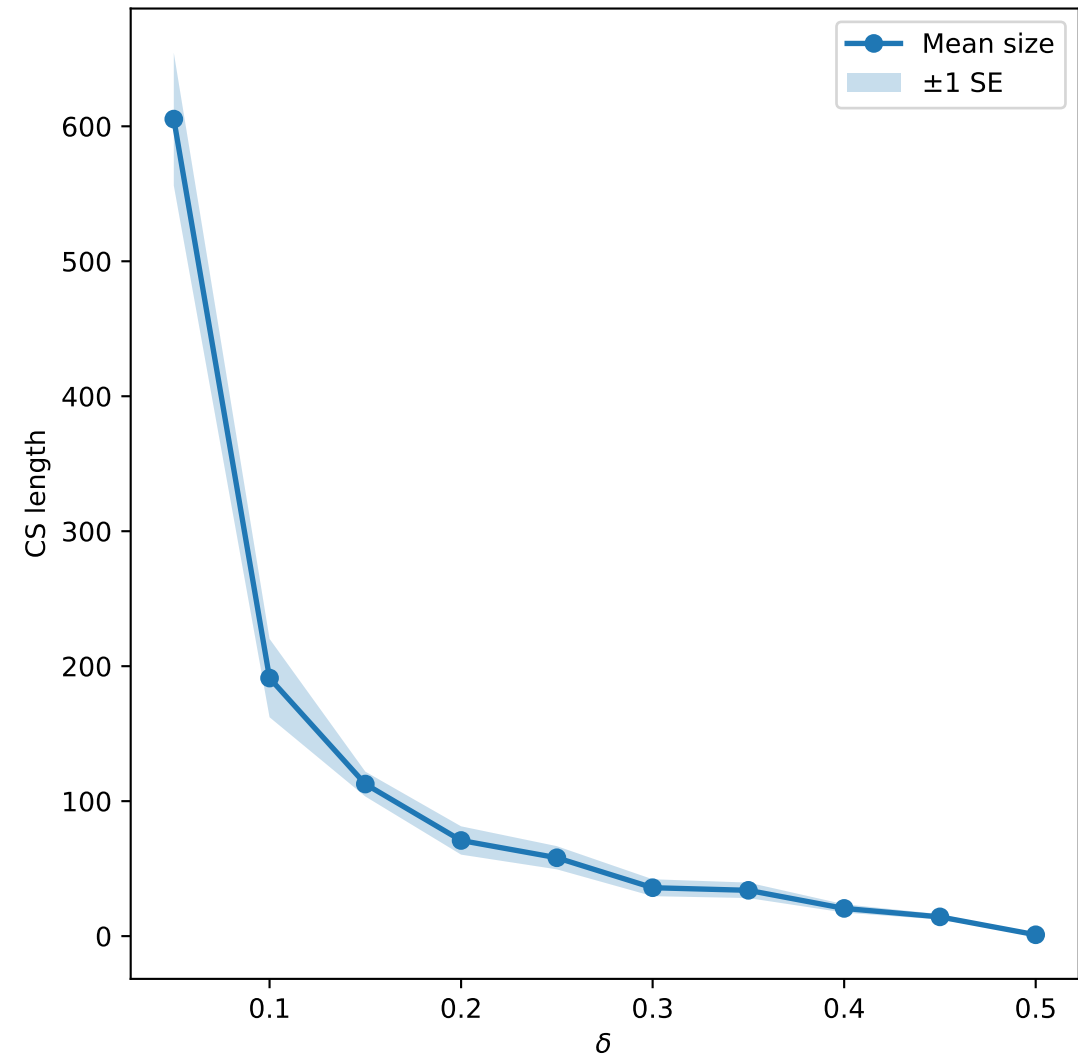
Confidence set size vs. \delta
