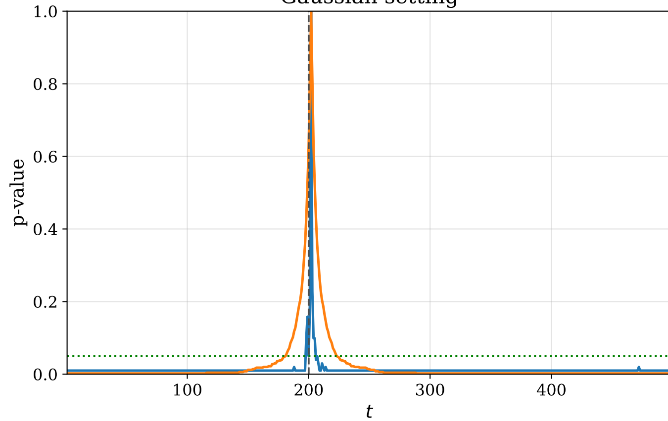
Gaussian setting
