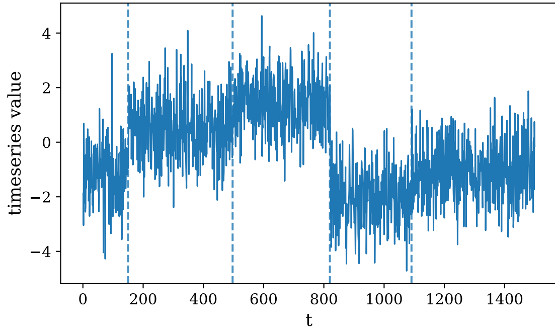
Time series
