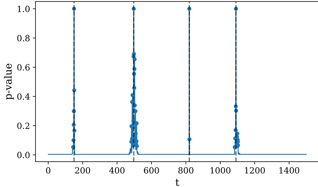
CONCH p-values
