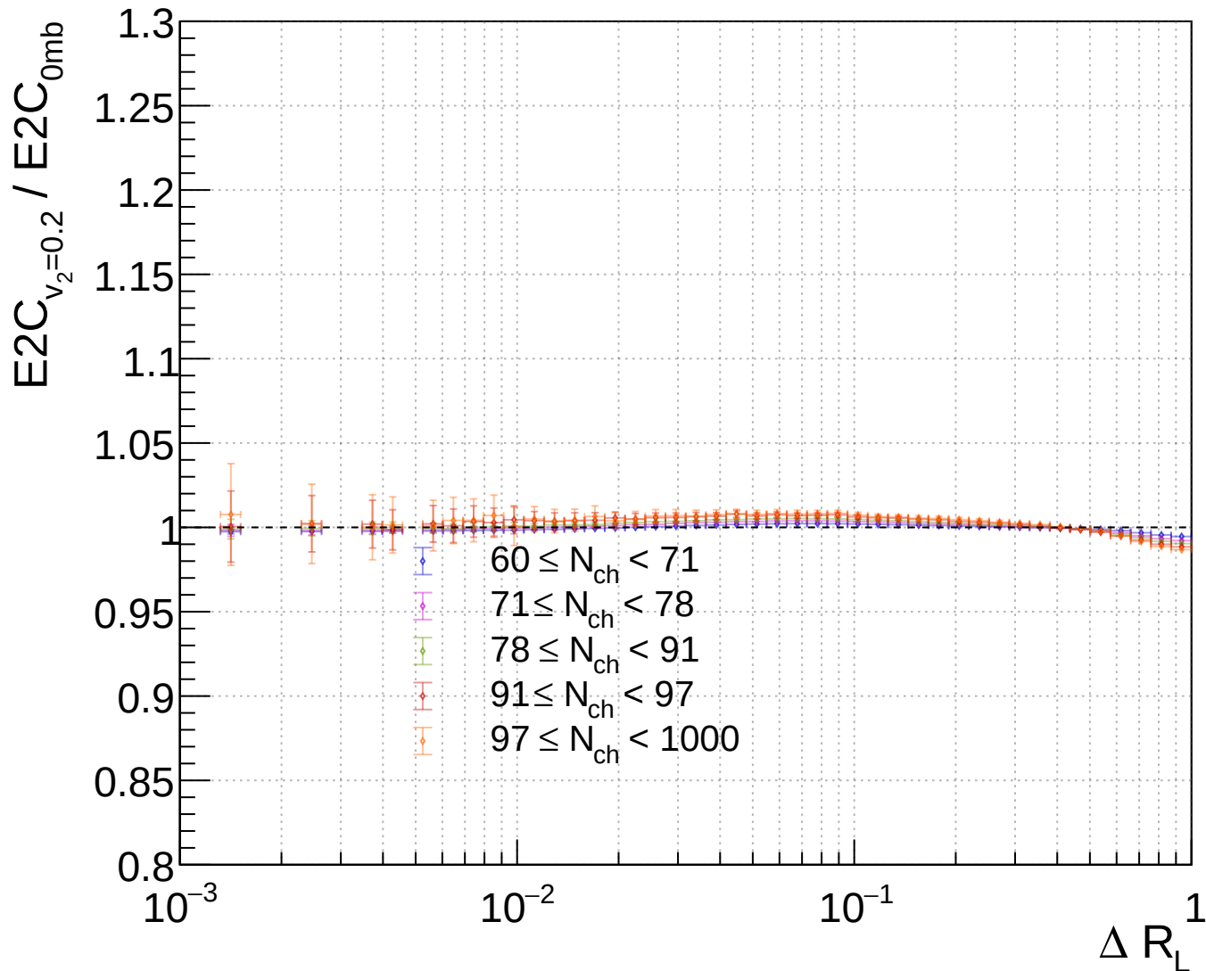
EEC ratio for high multiplicity bins ( v_2=0.2 )
