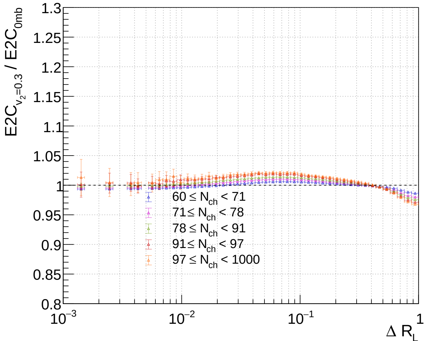
EEC ratio for high multiplicity bins ( v_2=0.3 )
