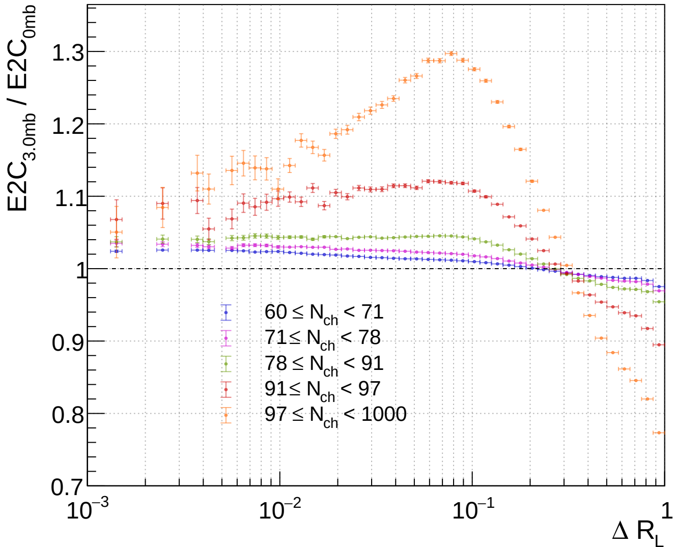
EEC ratio for high multiplicity bins (rebinned)
