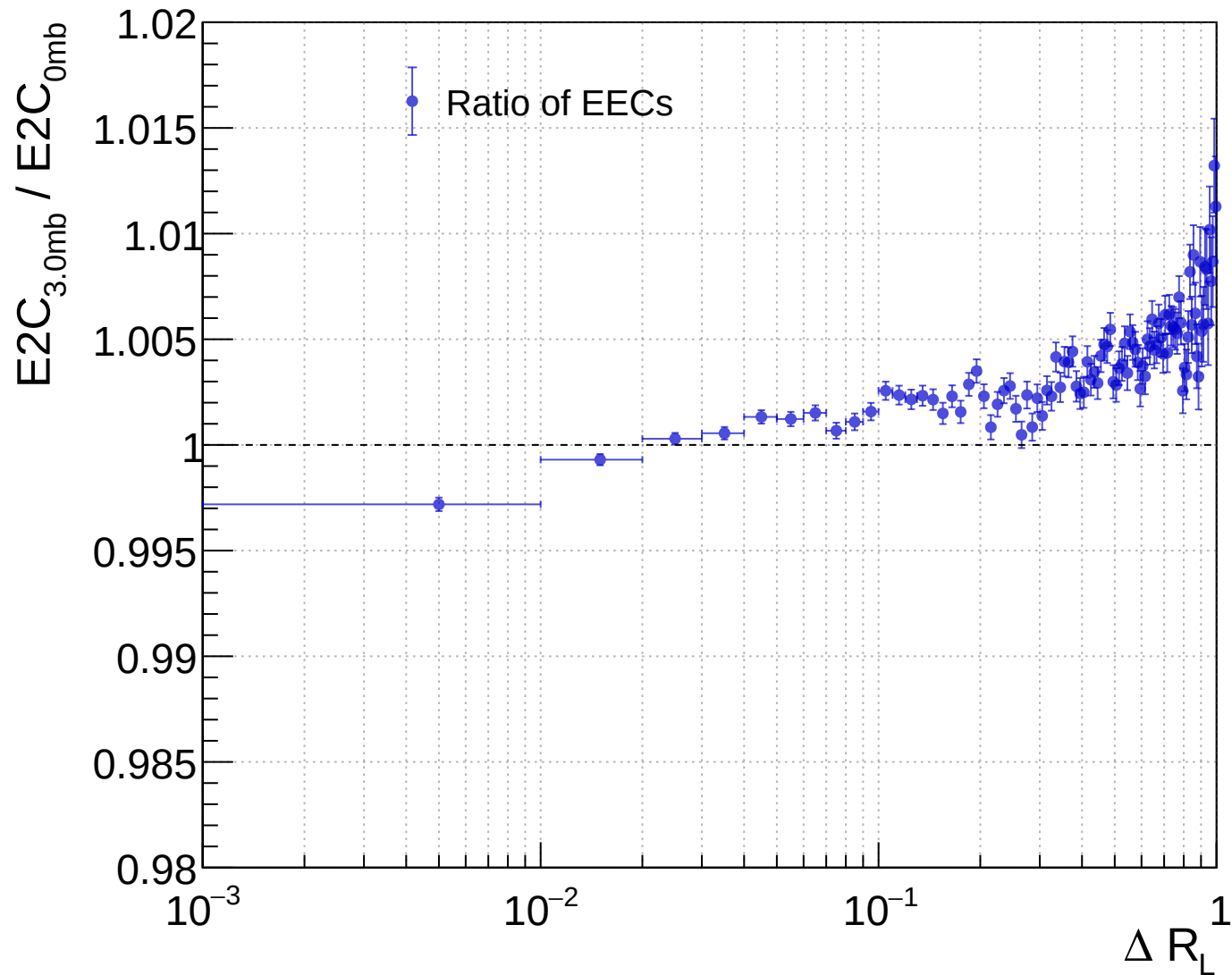
Ratio of EECs for inclusive datasets (rebinned)
