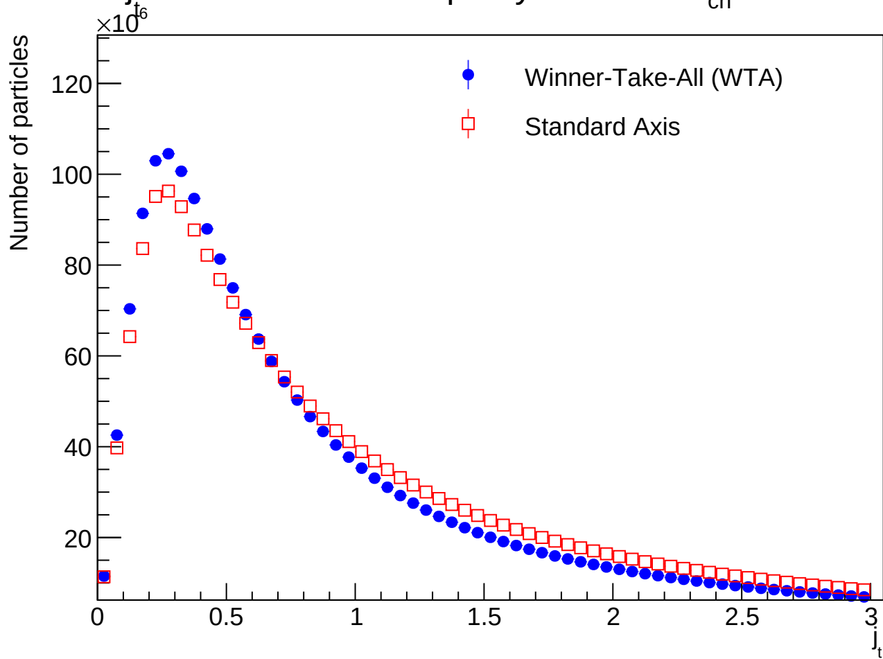
j_t distribution for multiplicity Bin: 60 \leq N_{ch} < 71
