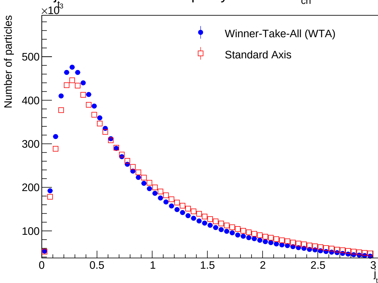
j_t distribution for multiplicity Bin: 91 \leq N_{ch} < 97
