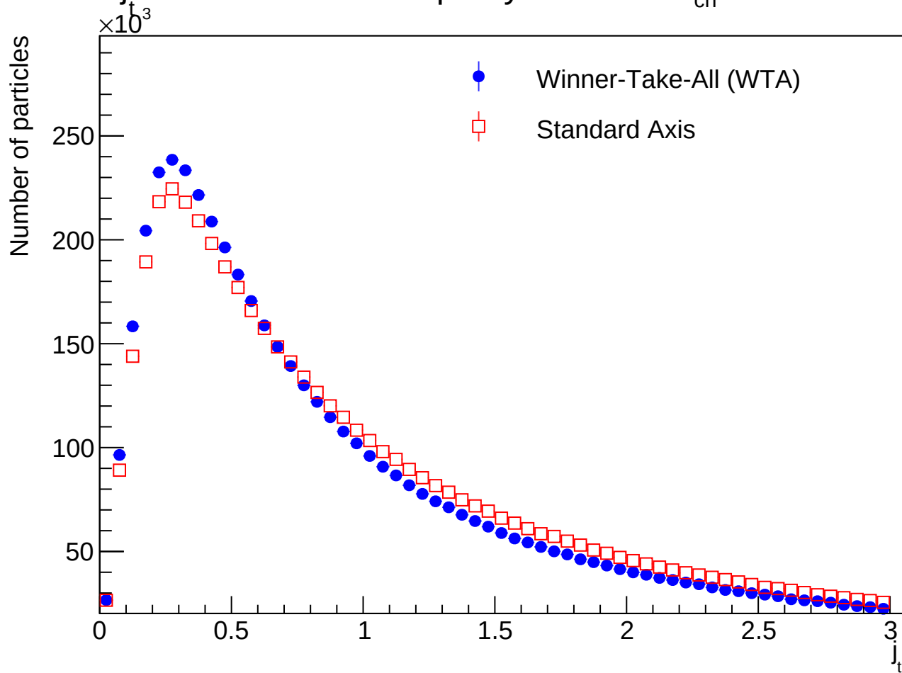
j_t distribution for multiplicity Bin: 97 \leq N_{ch} < 1000
