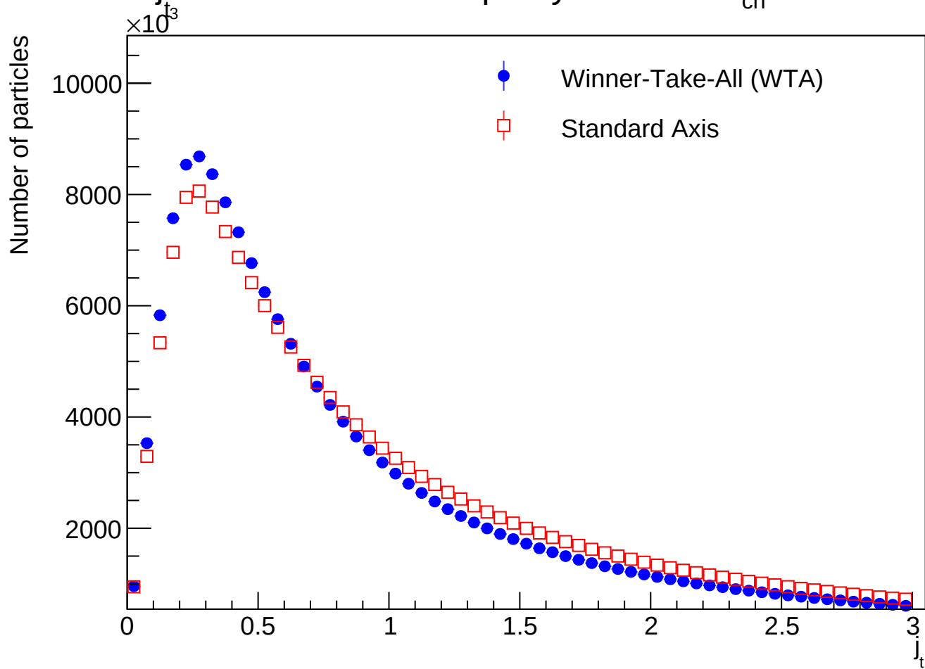
j_t distribution for multiplicity Bin: 71 \leq N_{ch} < 78
