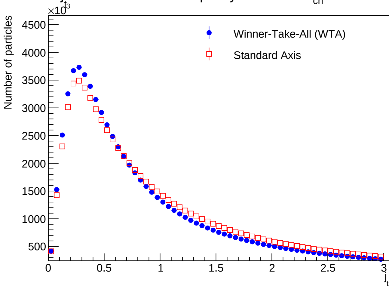
j_t distribution for multiplicity Bin: 78 \leq N_{ch} < 91
