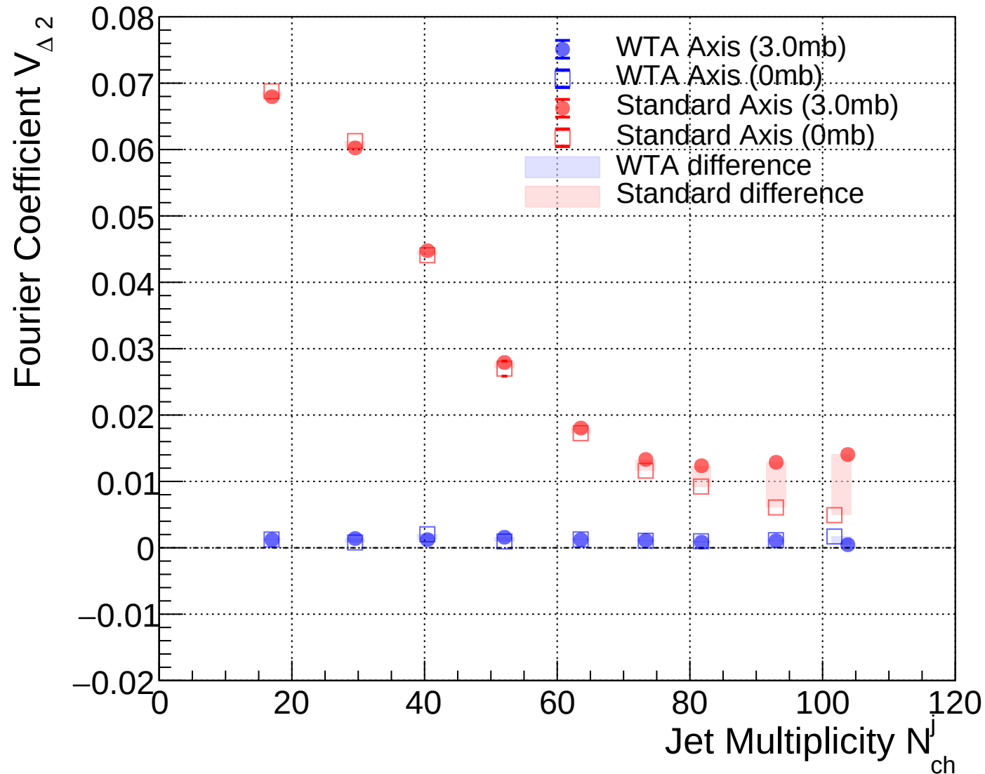
Fourier coefficients for data with and without hFSI
