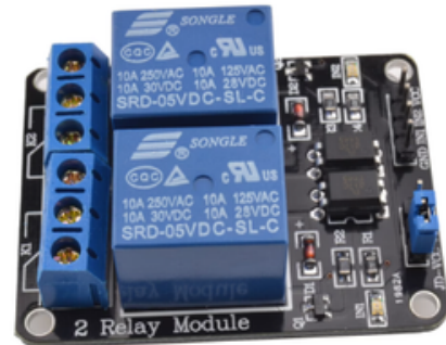
5V Dual Channel Relay Module
