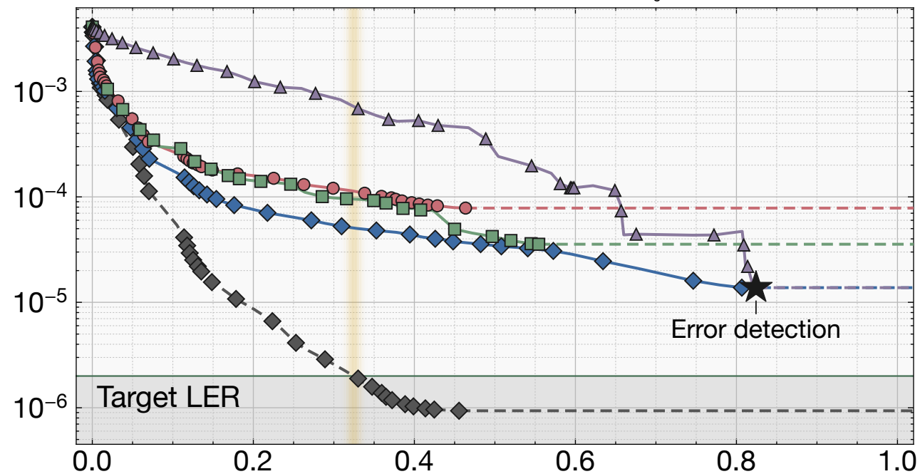
Surface code cultivation, f = 5
