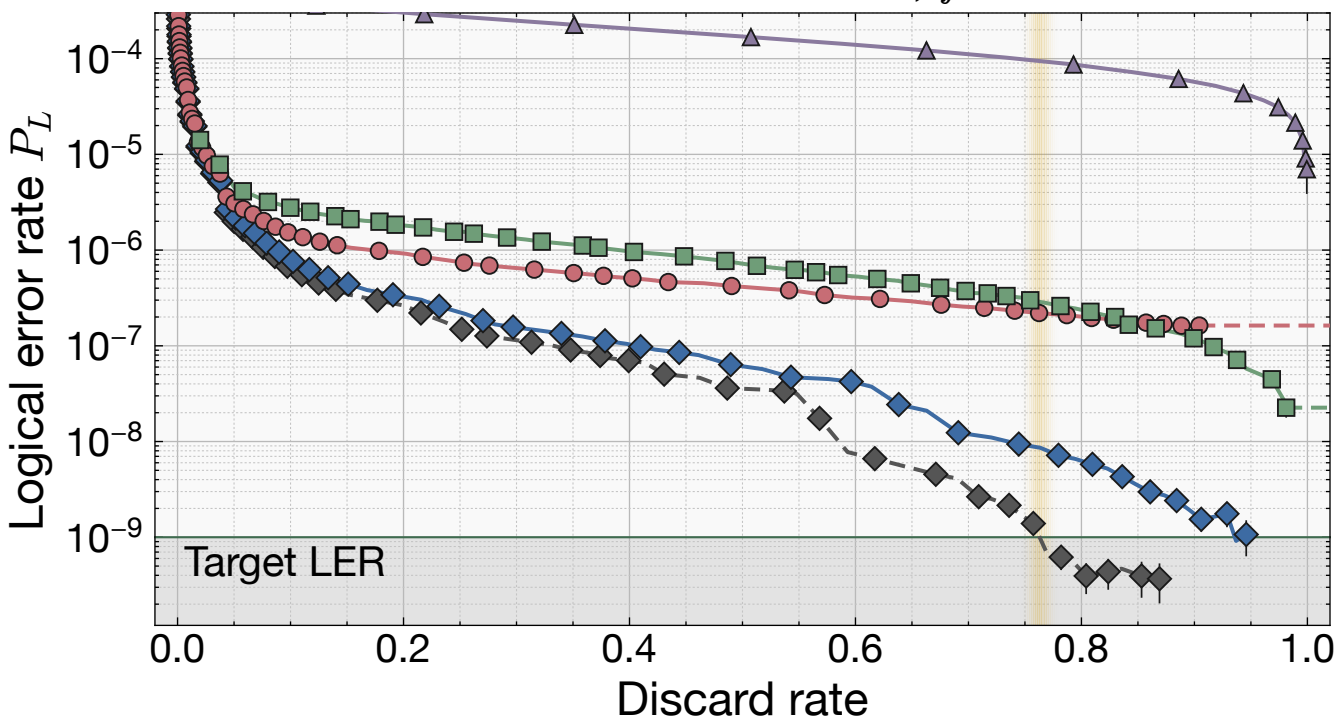
Color code cultivation, f = 5
