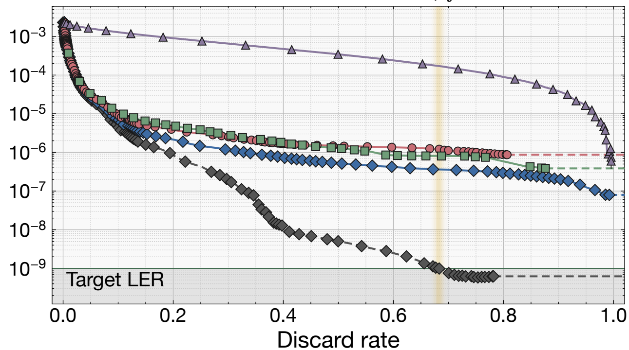
Surface code cultivation, f = 5
