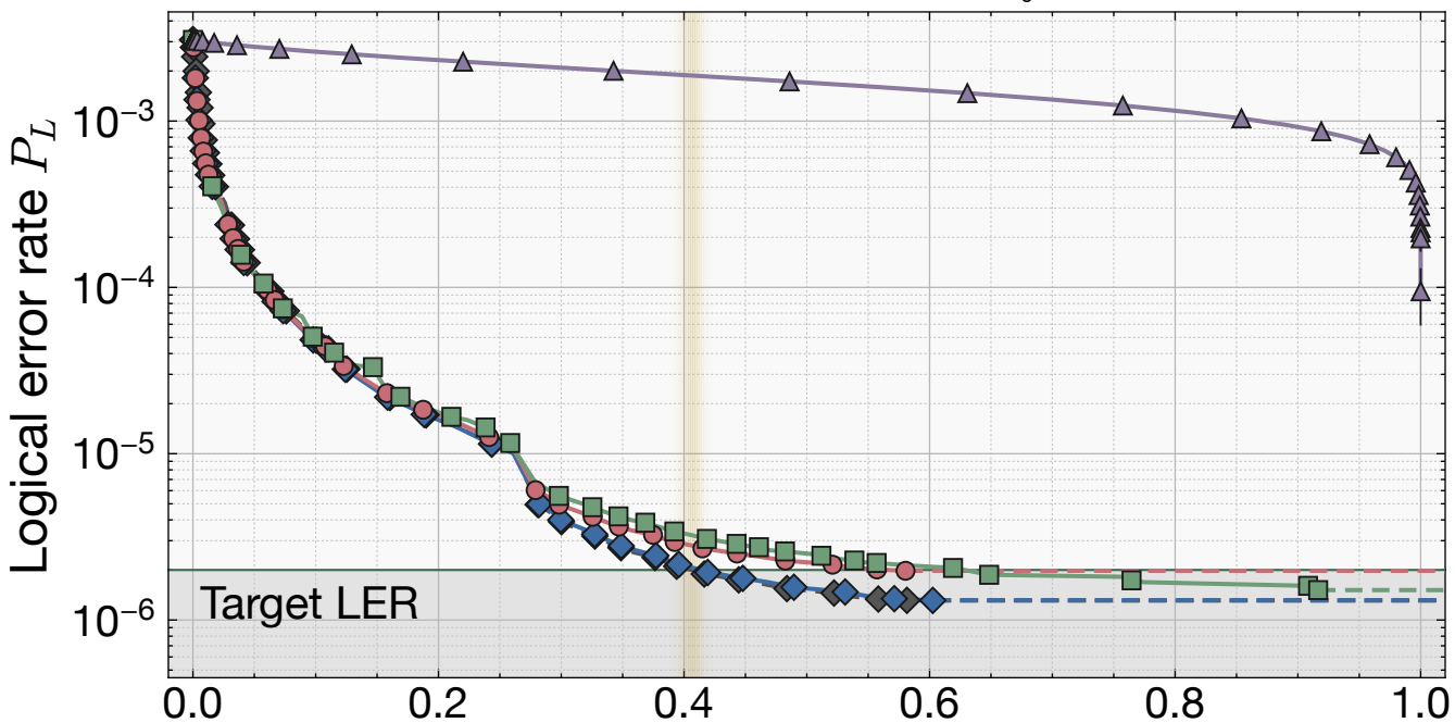
Color code cultivation, f = 5
