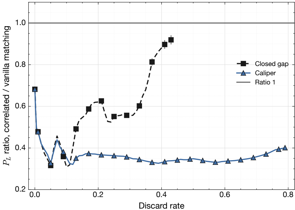
Surface code cultivation, f=3
