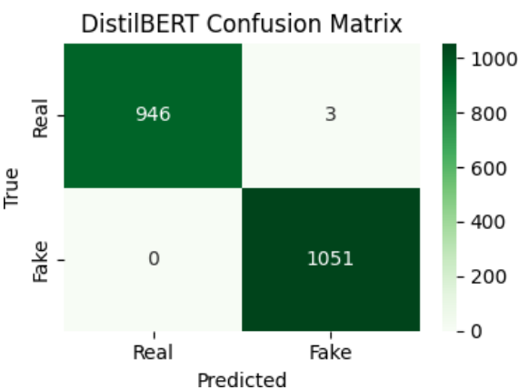
NLP Confusion Matrix
