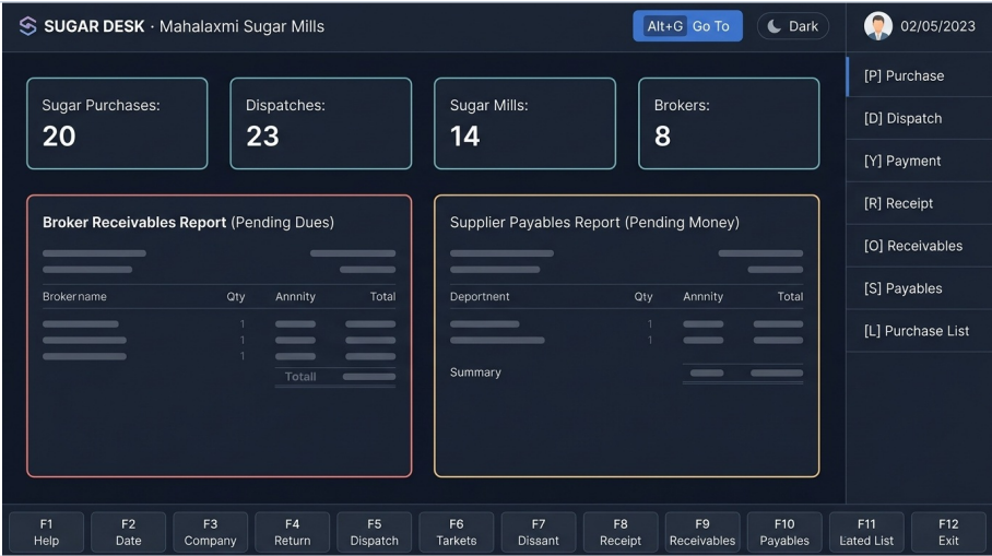
Figure 1: Sugar Desk Gateway Command Center with Live Transaction Counters & Pending Dues
