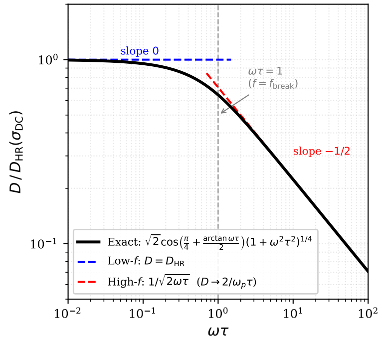
Universal Drude absorptance ratio
