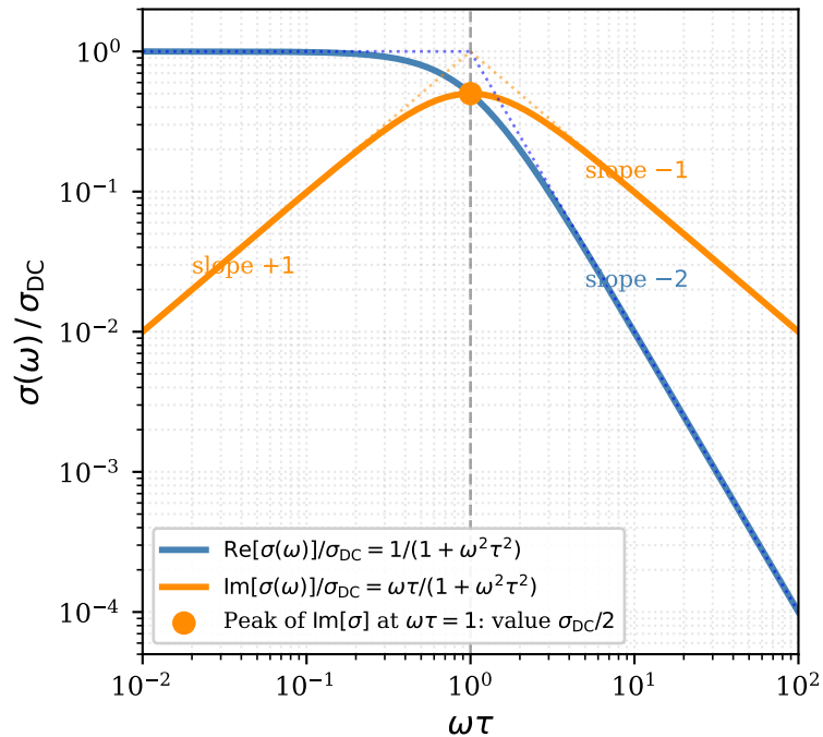
Drude AC conductivity
