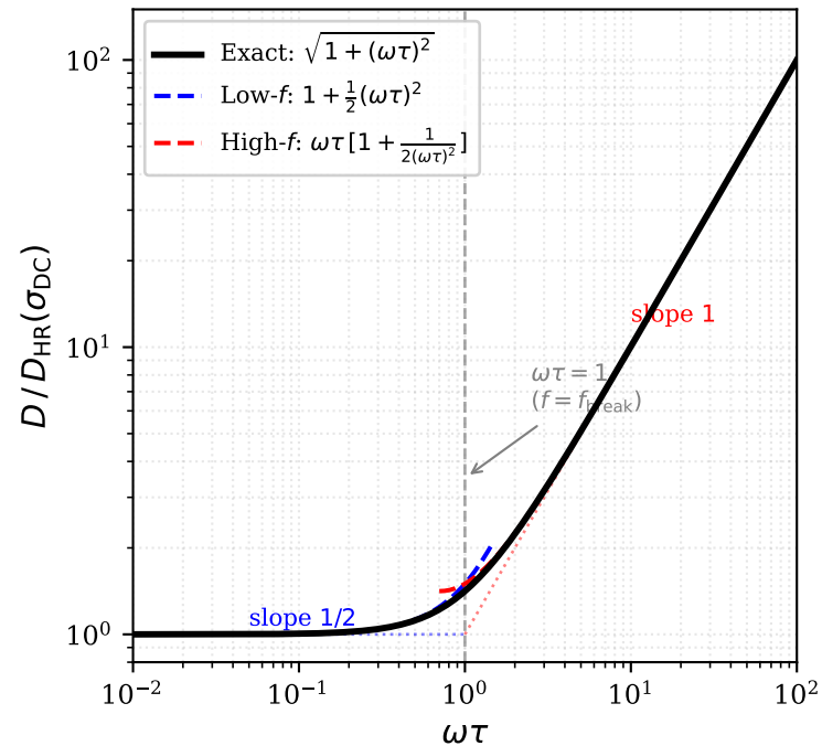
Universal Drude absorptance ratio
