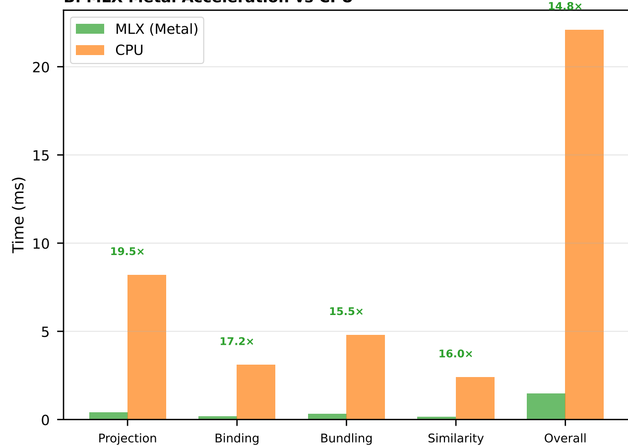
B. MLX Metal Acceleration vs CPU
