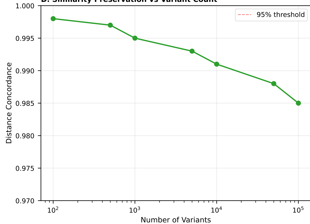
D. Similarity Preservation vs Variant Count
