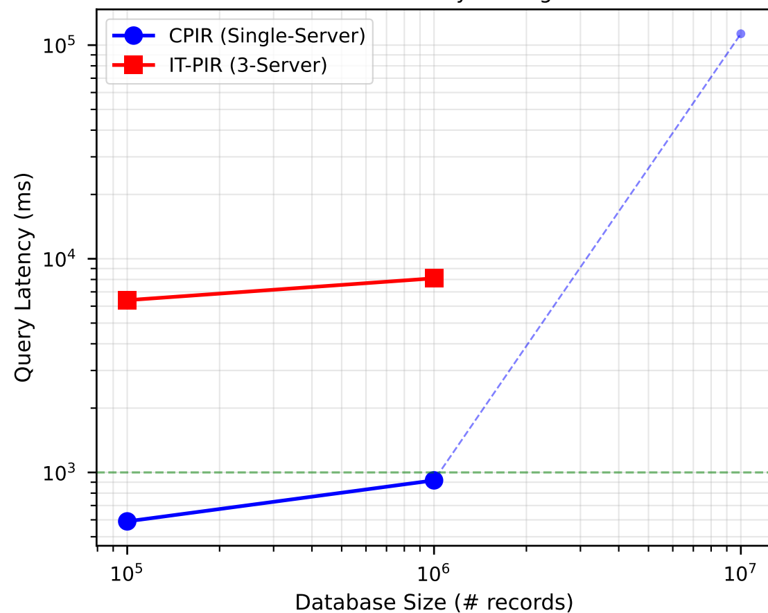
B. CPIR vs IT-PIR Trade-offs
