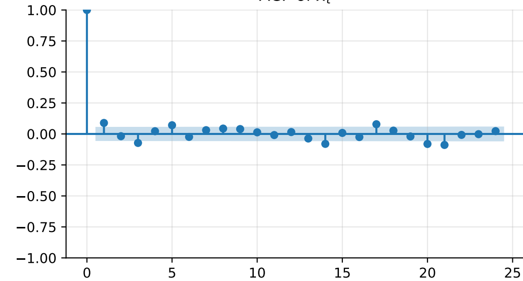
ACF of x_t
