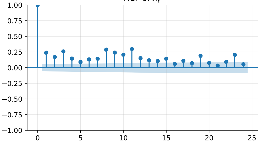
ACF of x_t^2
