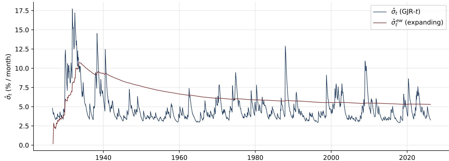
Conditional standard deviation: GJR- t vs.\ expanding-window benchmark
